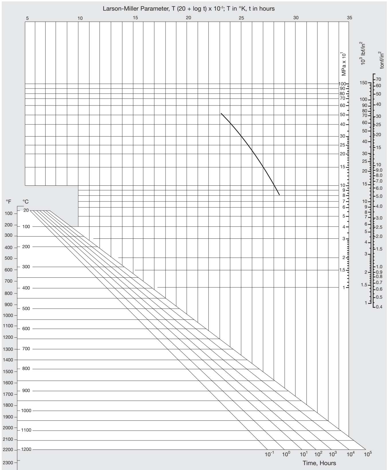
Figure 2. Creep-rupture properties of SOONV alloy 115 forged bar. Heat treatment 1.5 h/1190°C/AC+6h/1100°C/AC
