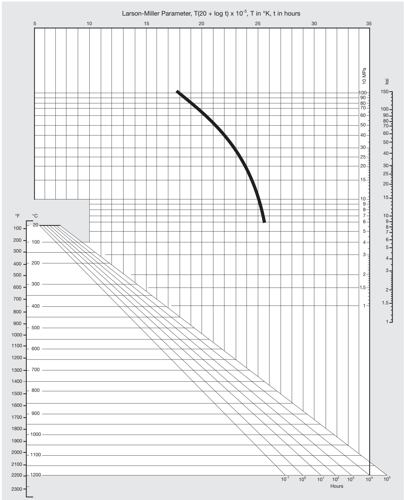
Figure 2. Creep-rupture properties of SOON alloy 901 forged bars.
