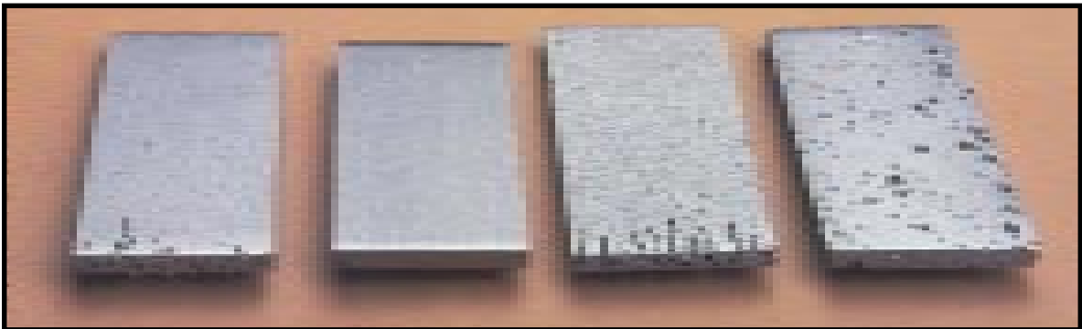
Samples were subjected to a solution of 11.5% H 2 SO 4 , 1.2% HCl, 1% FeCl 3 AND 1% CuCl 2 . Solutions for coupons 625 and C-4 were at 102°C, while C-276 and C-22 were at 125°C.
